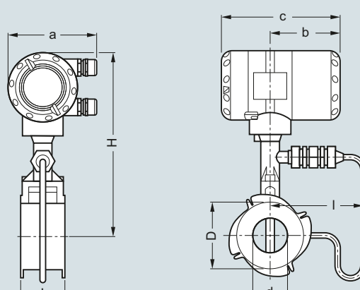
Sandwich version with pressure sensor
