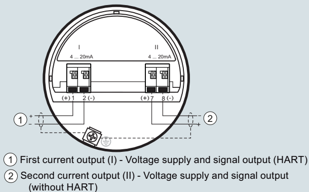
SITRANS LG series connections
