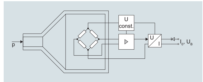
SITRANS P210 pressure transmitters (7MF1566-...), functional diagram
