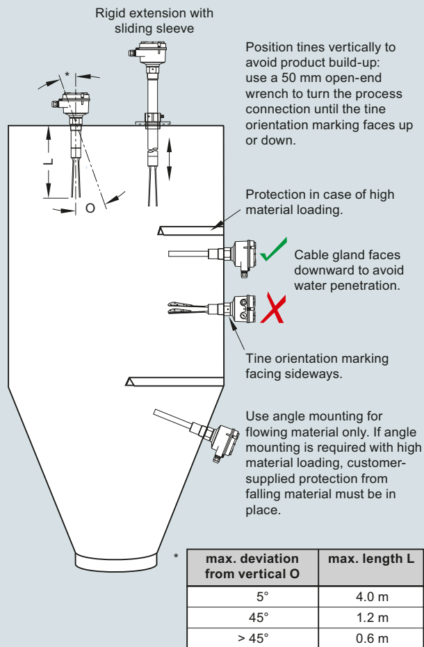
SITRANS LVS100 installation, dimensions in mm (inch)
