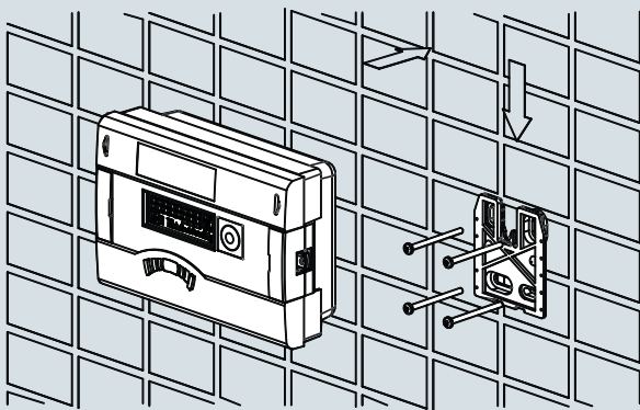
Wall mounting
