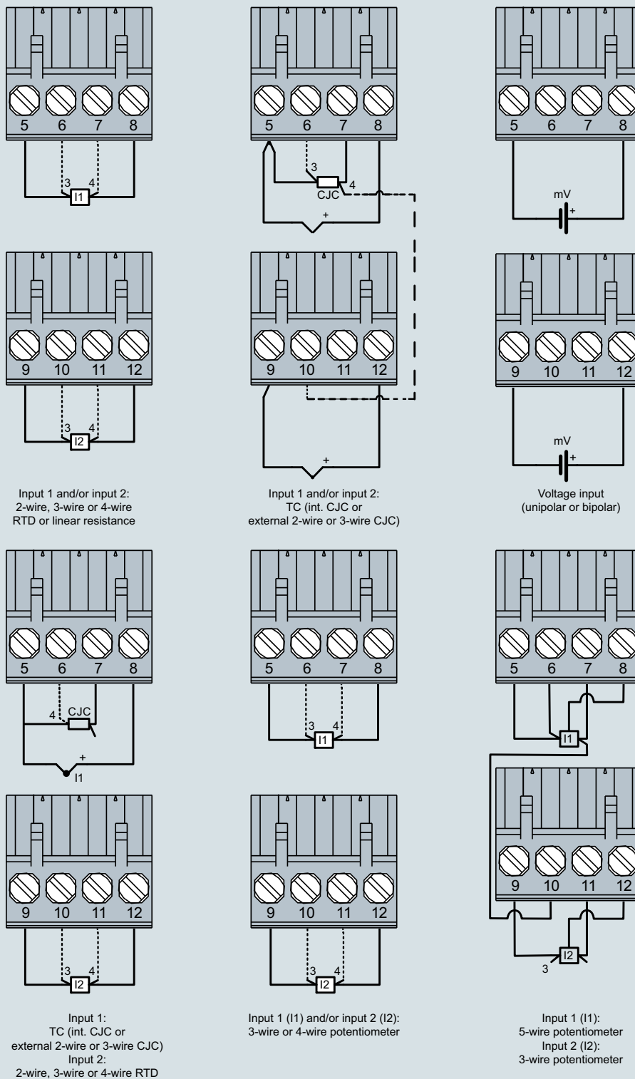
SITRANS TR420, input connection assignment
