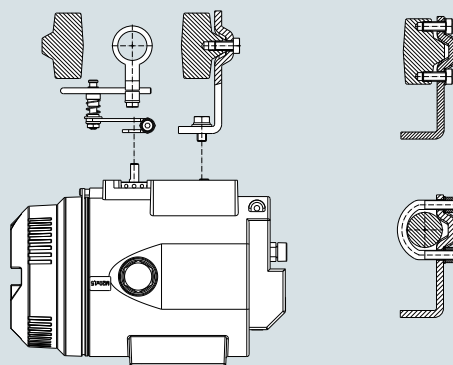
Mounting of SIPART PS2 in flameproof aluminum enclosure on linear actuators
