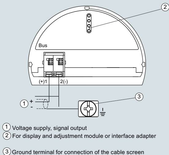
LG series connections
