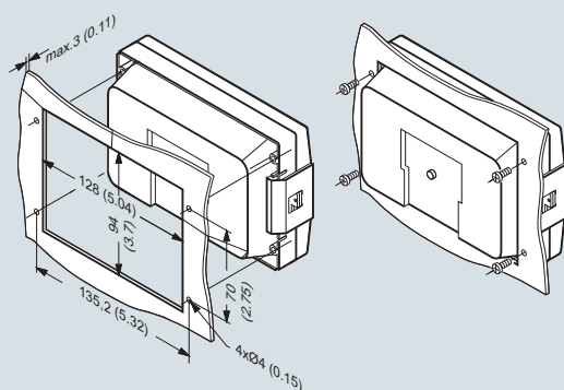
Panel mounting, dimensions in mm (inch)
