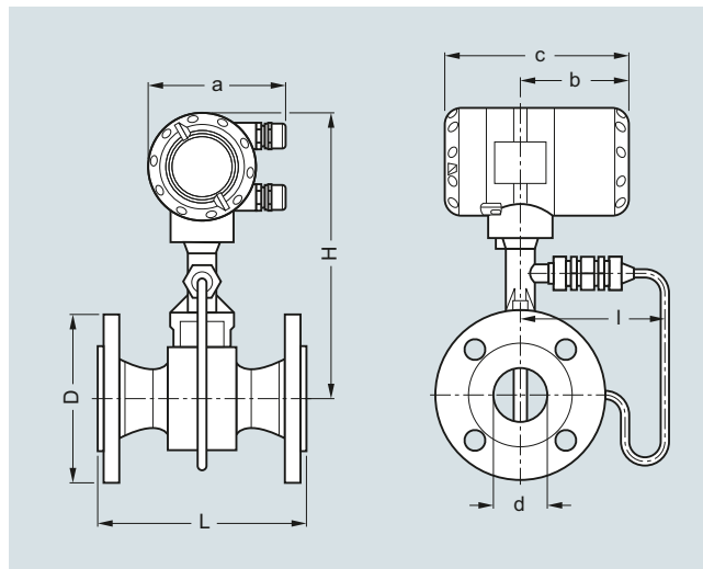
Flange version with pressure sensor
