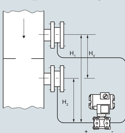
Installation type D Filter monitoring
